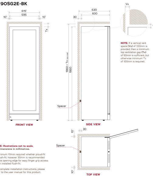
170 Bottle Wine Cabinet V190SG2E-BK
